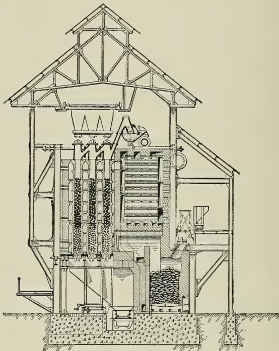
FIG. 88.—Vertical Gas-Works Retort.
